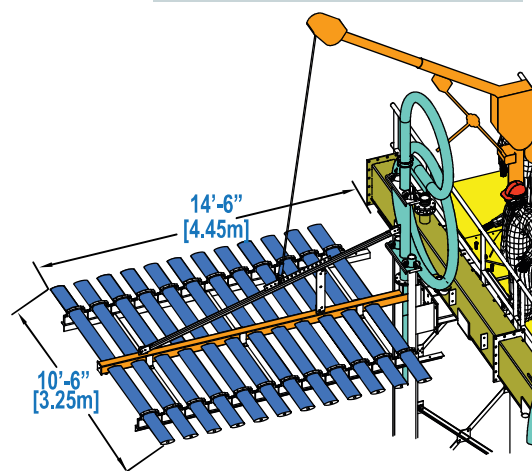
Oxidation Ditch - Retrofit
