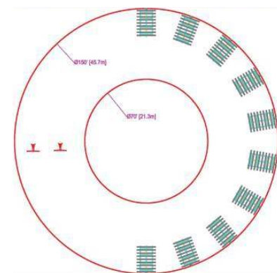
Concentric Ring Aeration Basin
