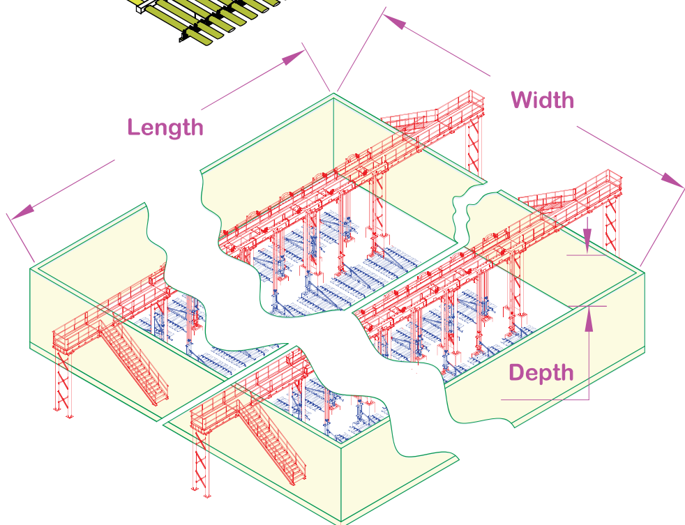
Rectangular Aeration Basin
