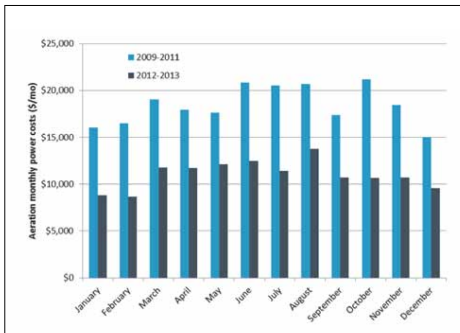
Figure 2. Muddy Creek aeration power costs
