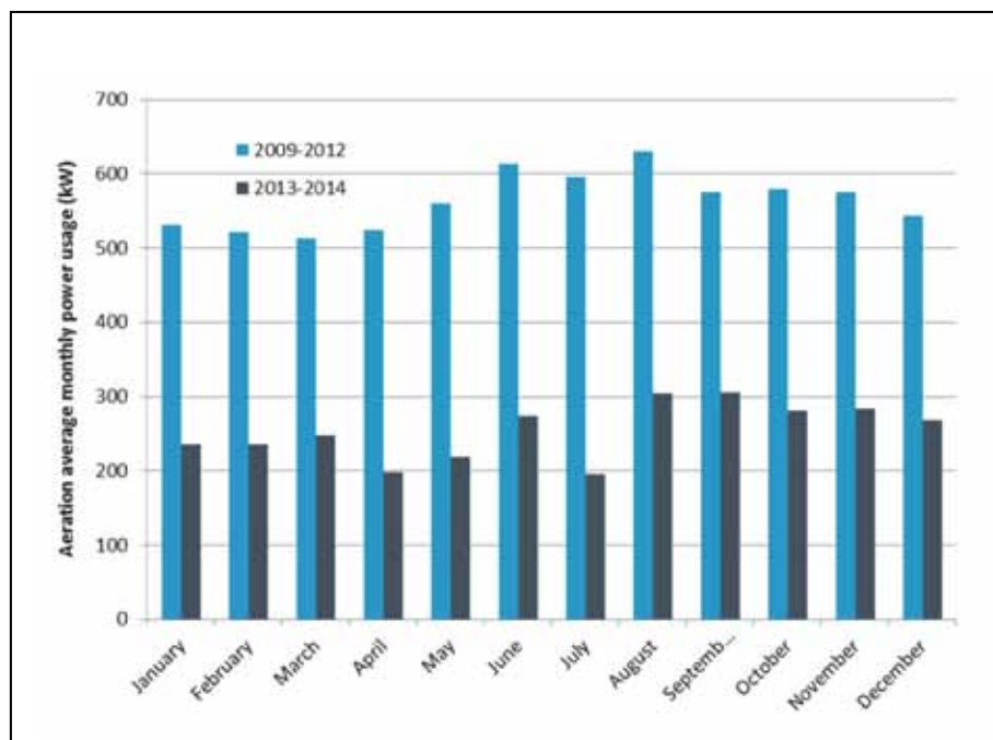
Figure 1. Little Miami aeration power usage
